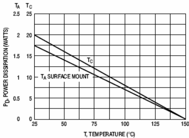
Figure 1. Power Derating
